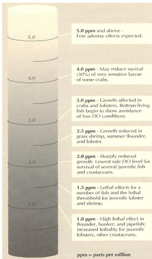
Effect of DO on marine life. (Source: Hempstead Harbor, Its History, Ecology, and Environmental Challenges, 1998)
